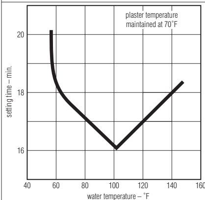
Fig. 1—Effect of slurry temperature on setting time.
